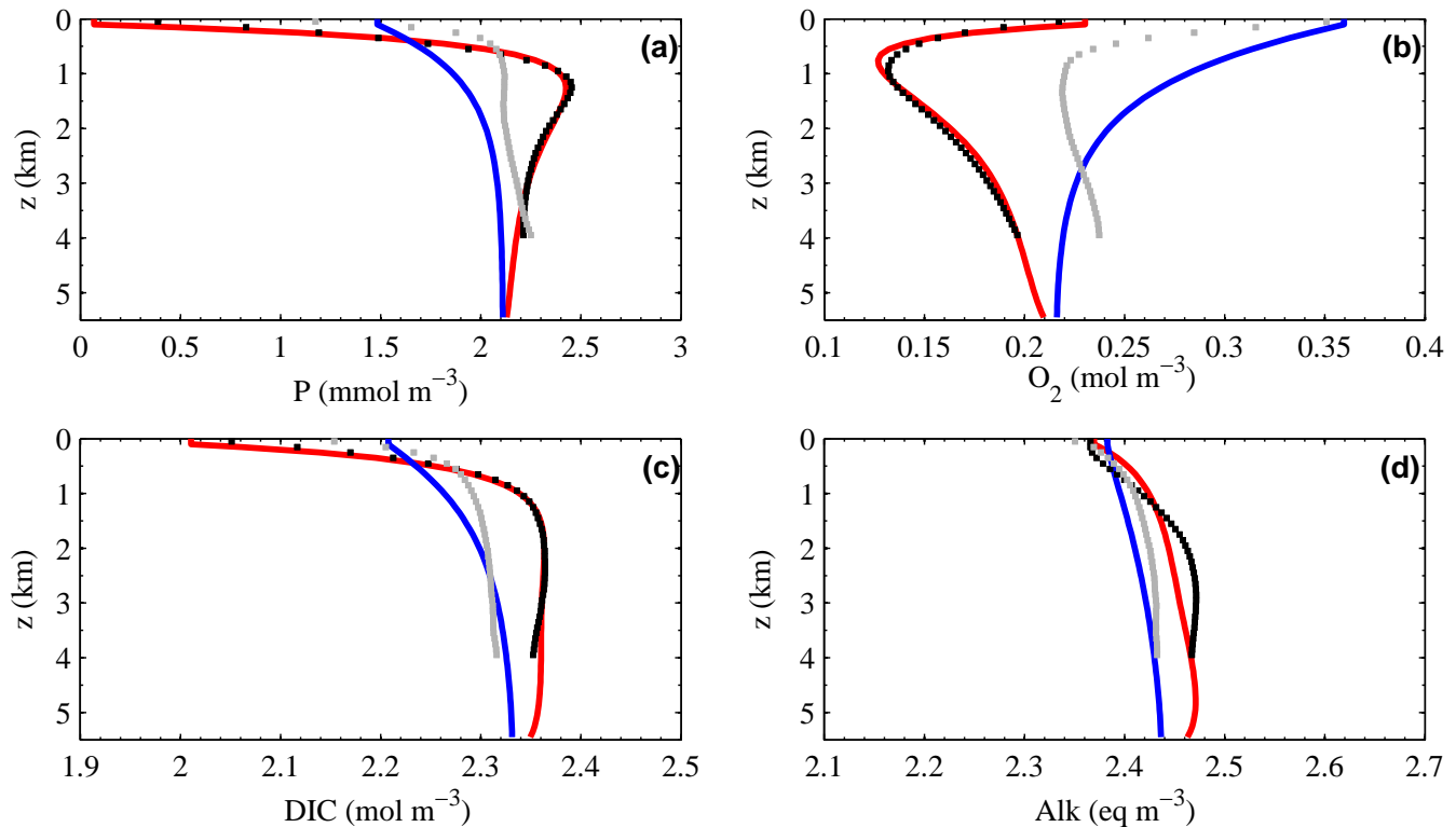
Fig. 4. Steady state, pre-industrial simulations (solid lines) compared to data (dots) of mean ocean profiles of (a) phosphate (P), (b) dissolved oxygen ( \text{O}_2 ), (c) dissolved inorganic carbon (DIC) and (d) alkalinity (ALK). Low-mid latitude and high latitude simulations are given in red and blue, respectively. Mean, data-based profiles from the low-mid and high latitude sectors are given in black and grey, respectively. These profiles have been calculated from GEOSECS data as in Shaffer and Sarmiento (1995) and Shaffer (1996).
